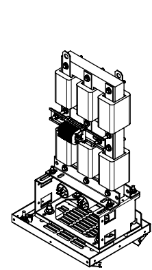
ISOMETRIC VIEW (PANELS REMOVED)
